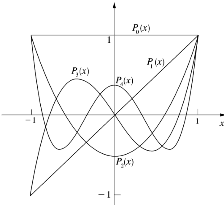
Figure 4.1 Legendre's polynomials.
