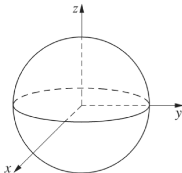
Figure 4.3 Spherical capacitor.
