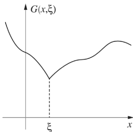
Figure 2.3 Green's function.
