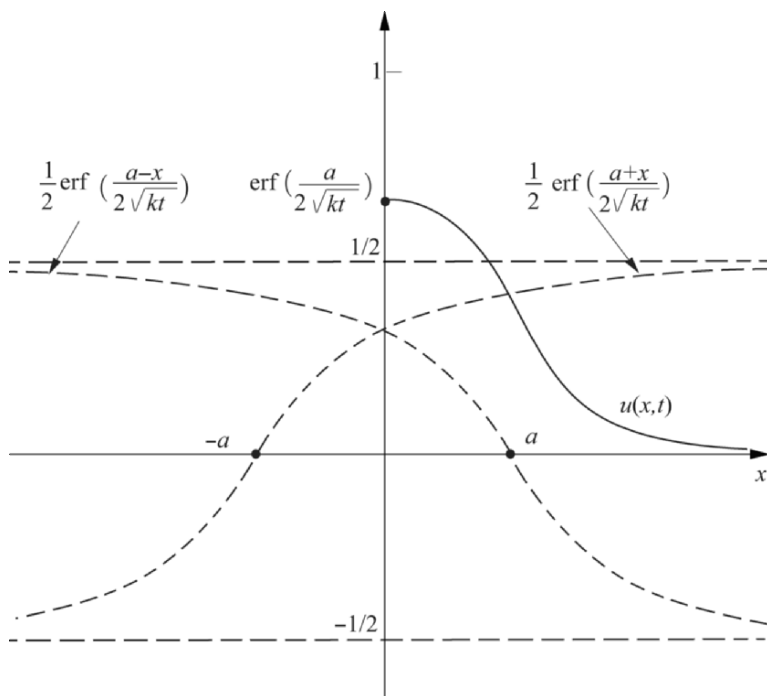
Figure 6.5 Temperature distribution on a semi-infinite rod.
