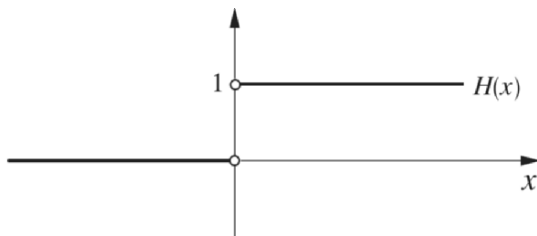
Figure 7.1 The Heaviside function.
